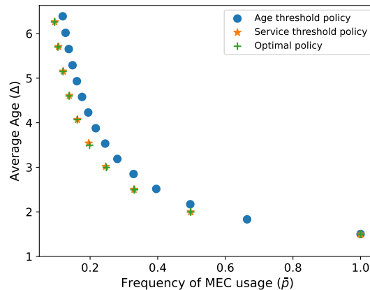
Fig. 5. Age vs. frequency of using the MEC for \mu = 0.01 . a^* varies from 1 to 15 for the age threshold policy, and z^* varies from 0 to 9 for the service threshold policy. For the optimal policy, \lambda \in (0, 50) .
